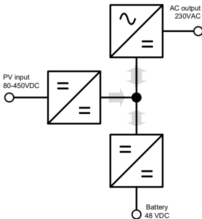
Inverter RS Smart Solar 48/6000
