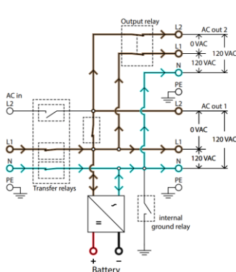
Vermogenstroom, 120 VAC-invoer
