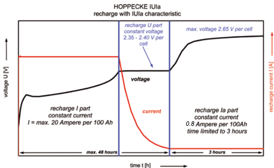
Fig. 9-2: IUla characteristic
