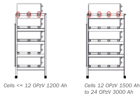
Fig. 5-12: Example of a horizontal arrangement of the batteries with OPzV-cells in a battery cabinet
