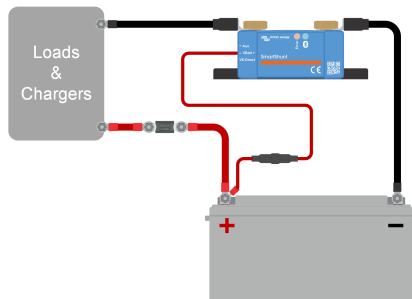
Installatie basis accumonitor.
