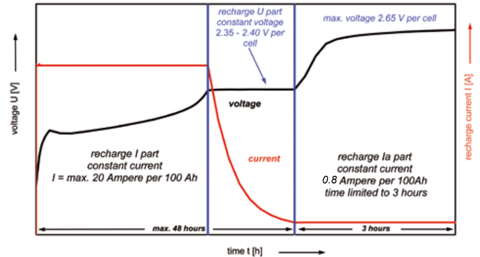
Fig. 9-2: IUa characteristic
