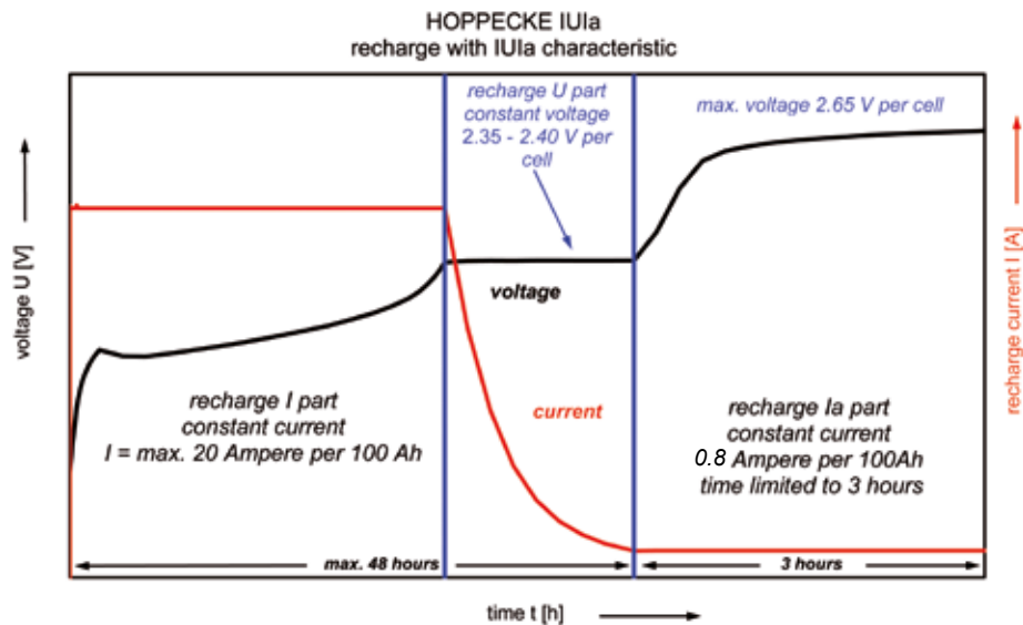
Fig. 9-2: IUa characteristic
