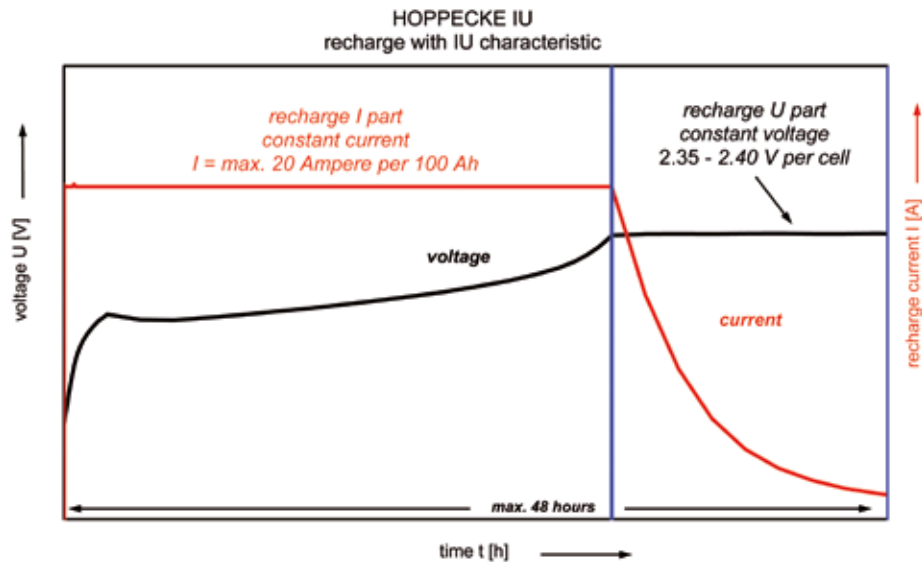
Fig. 9-1: IU characteristic
